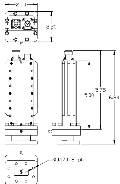
LNA with optional Input Isolator
