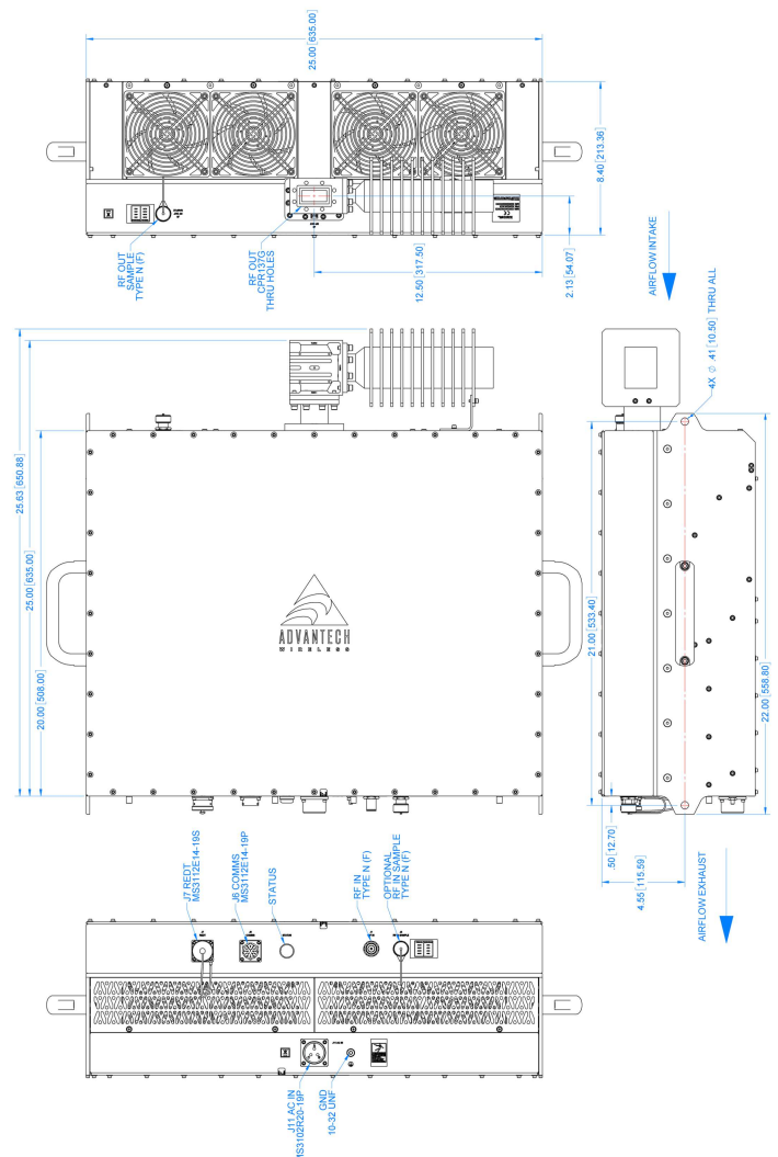
800W C-Band SSPB
