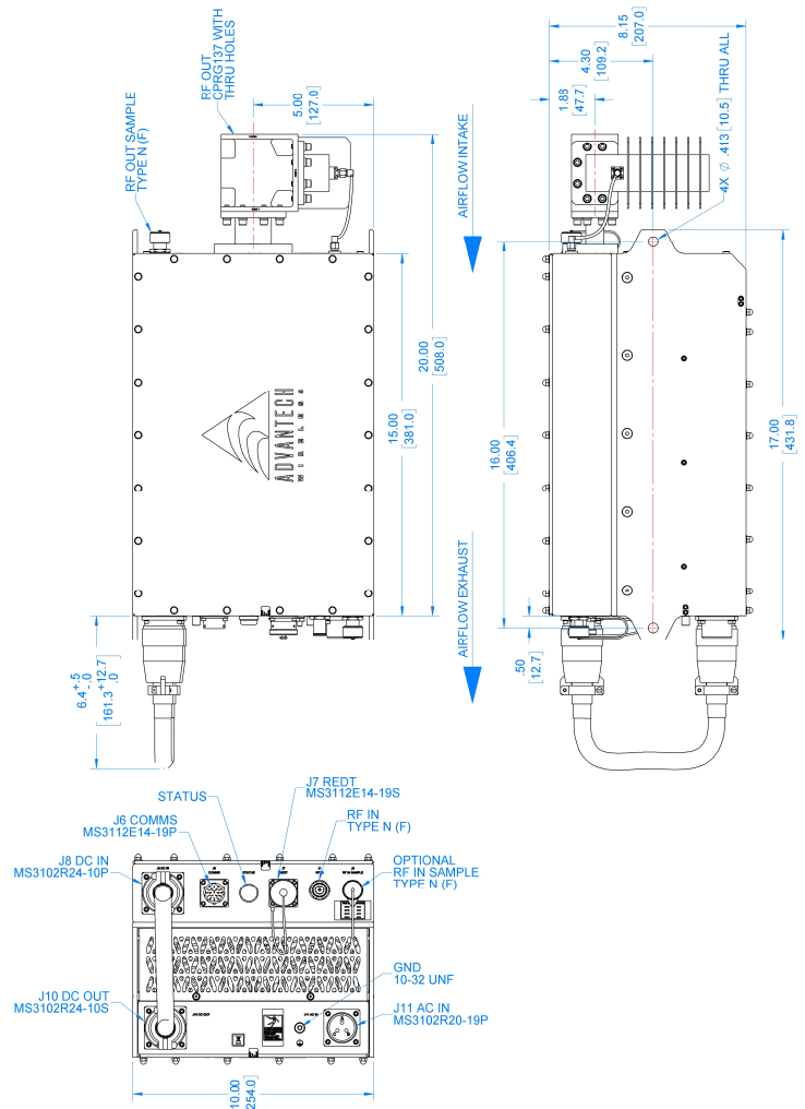
400W C-band GaN SSPB
