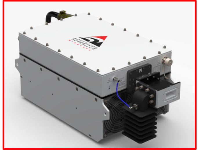
400W C-band GaN SSPB
